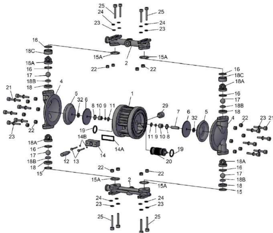
Spare Part List Drawing Ruby 115 AISI 316
