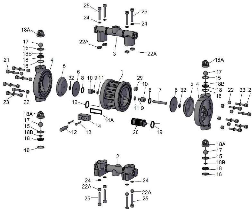
Spare Part List Drawing Ruby 015 Non Metallic
